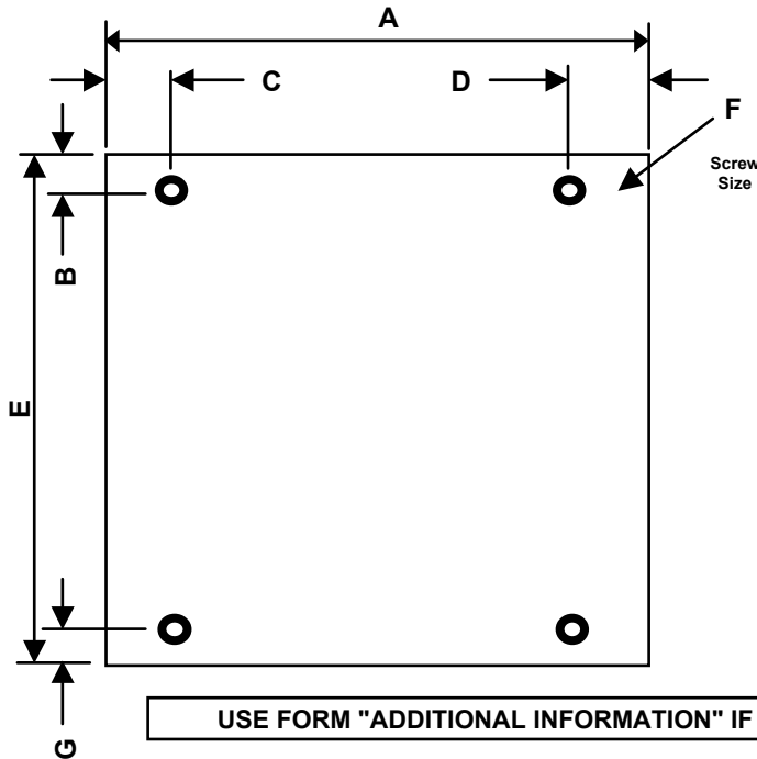
Existing Faceplate Dimensions
